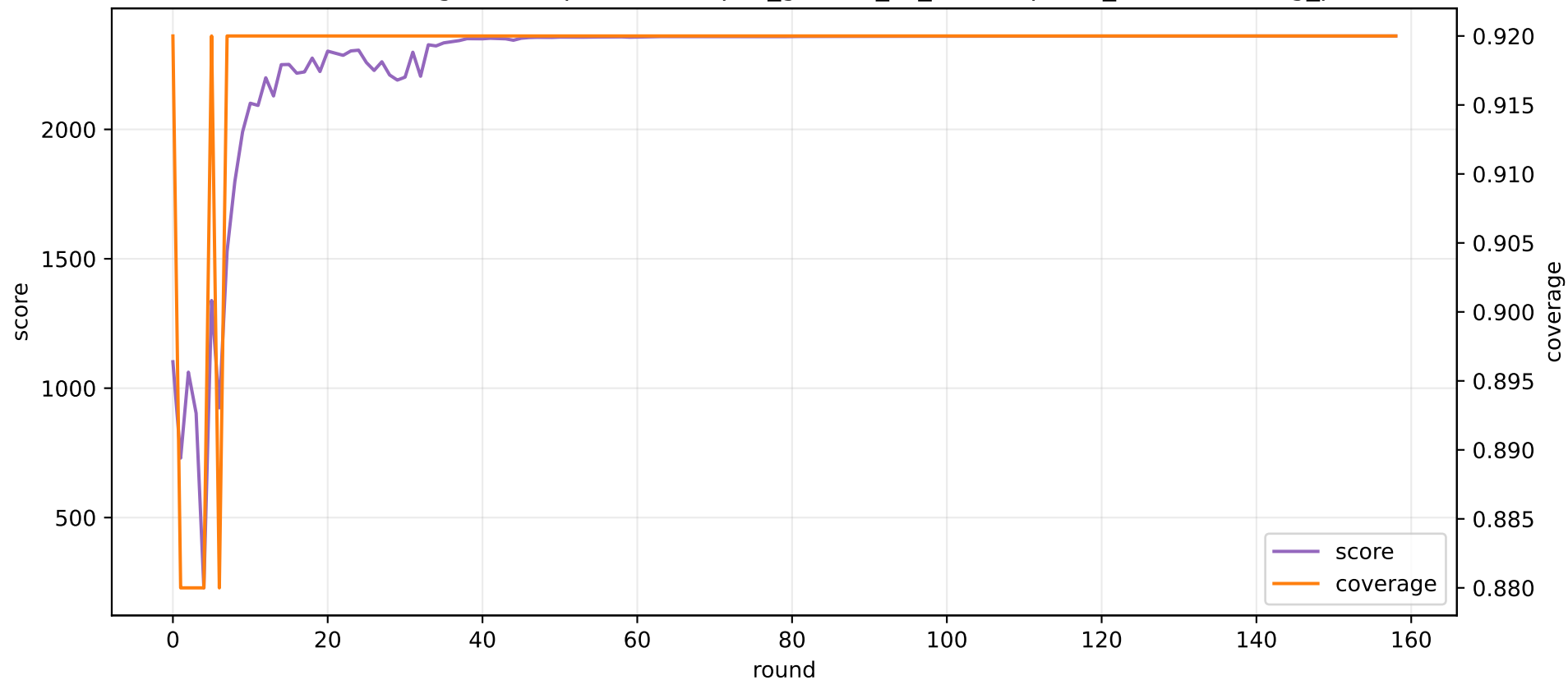
ASA score/coverage trace: pair 4 Grampus_griseus_vs_Globicephala_melas existing_paf
