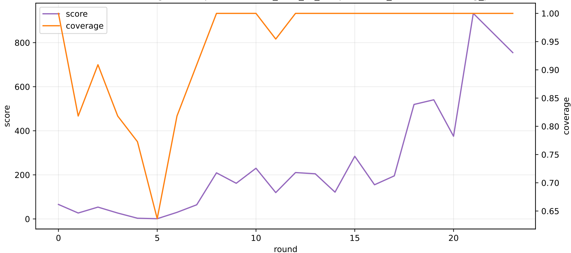
ASA score/coverage trace: pair 7 Orcinus_orca_vs_Neophocaena_sunameri existing_paf
