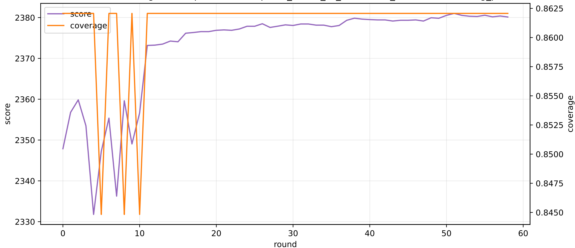
ASA score/coverage trace: pair 5 Globicephala_melas_vs_Pseudorca_crassidens existing_paf
