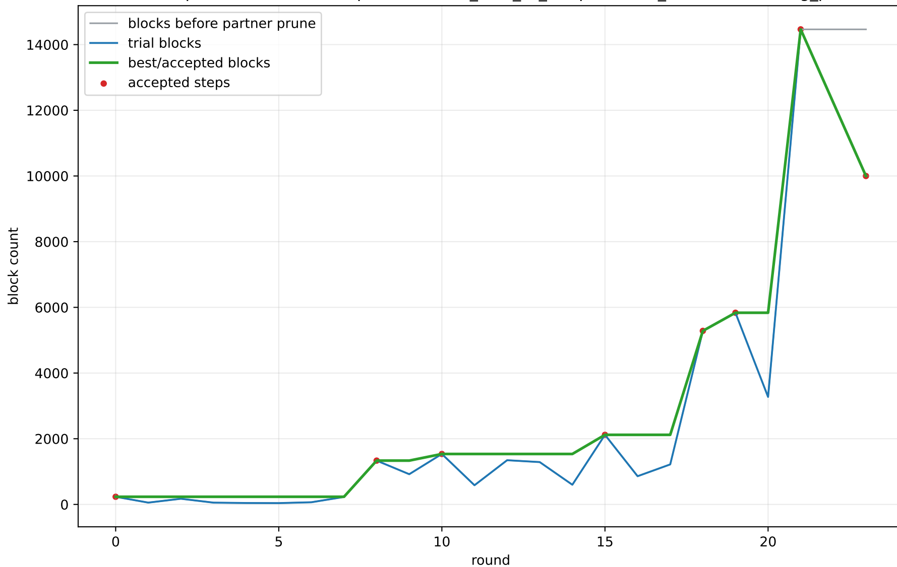
ASA optimizer block trace: pair 7 Orcinus_orca_vs_Neophocaena_sunameri existing_paf
