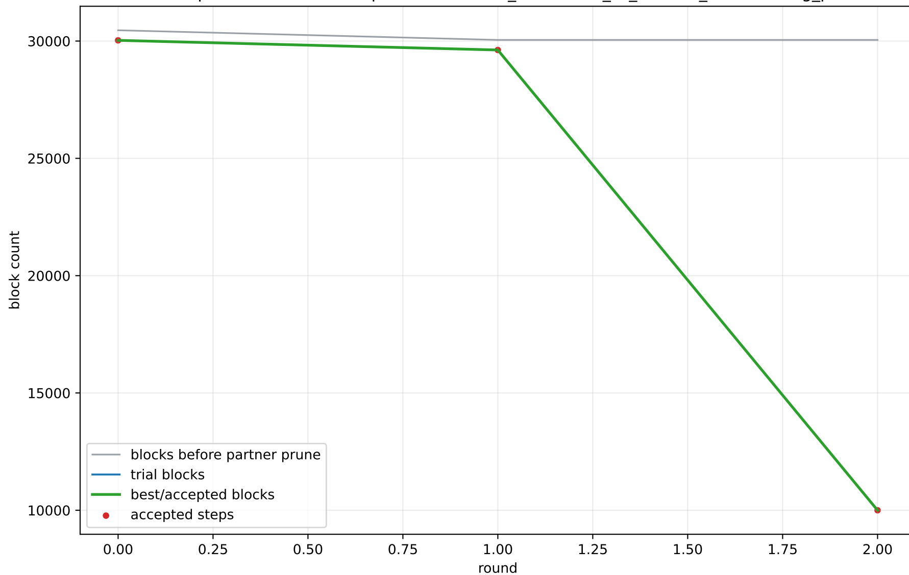
ASA optimizer block trace: pair 6 Pseudorca_crassidens_vs_Orcinus_orca existing_paf
