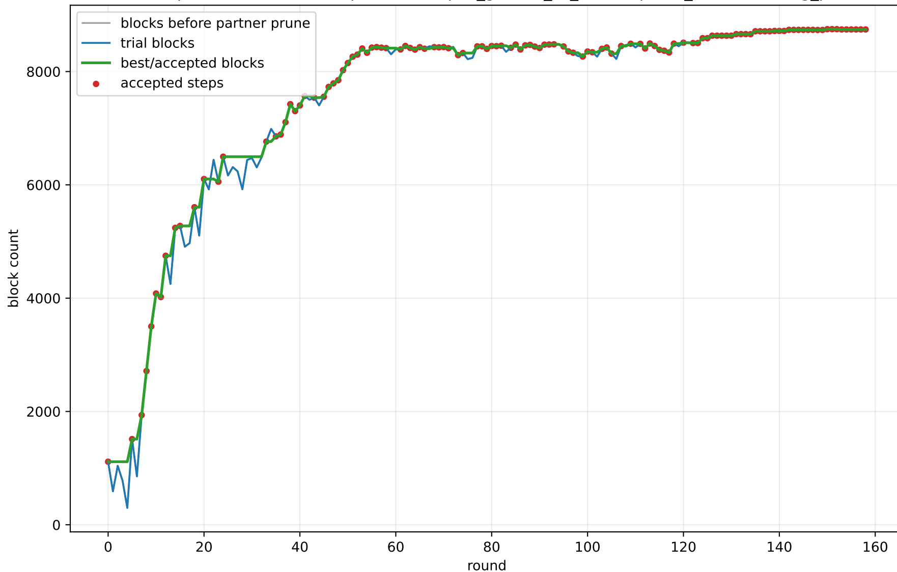
ASA optimizer block trace: pair 4 Grampus_griseus_vs_Globicephala_melas existing_paf
