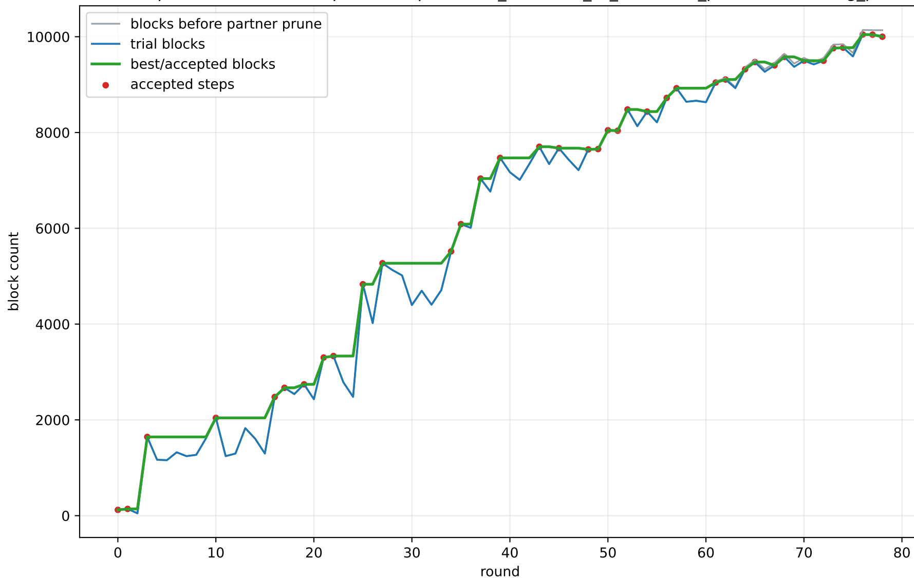
ASA optimizer block trace: pair 8 Neophocaena_sunameri_vs_Phocoena_phocoena existing_paf
