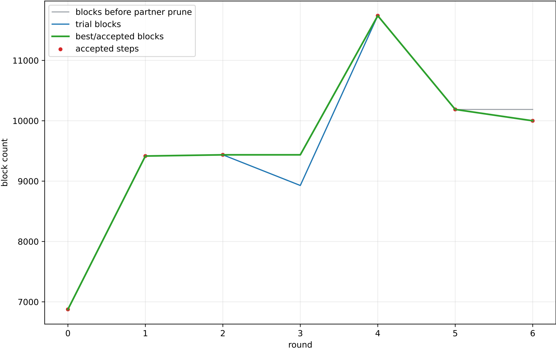
ASA optimizer block trace: pair 2 Lagenorhynchus_albirostris_vs_Lagenorhynchus_acutus existing_paf
