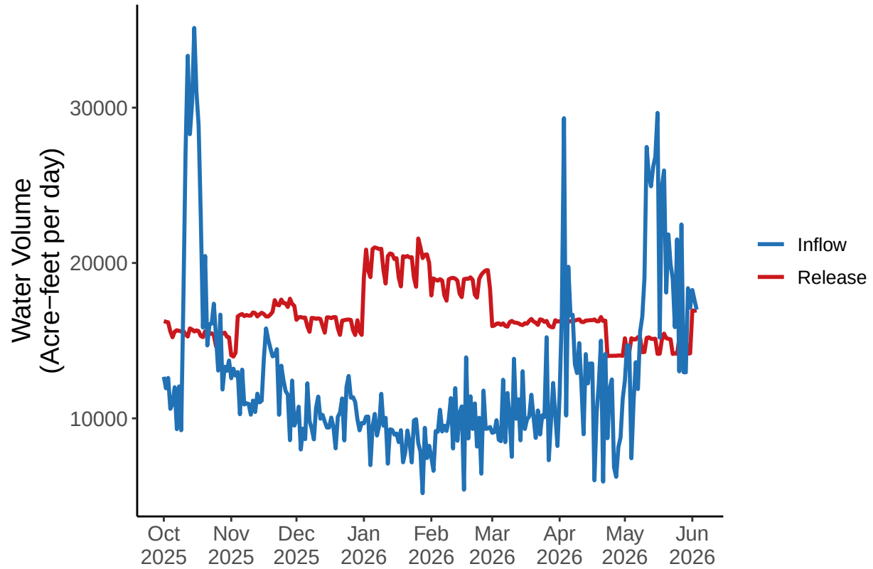
Figure 6B: Lake Powell Daily Inflow and Release
