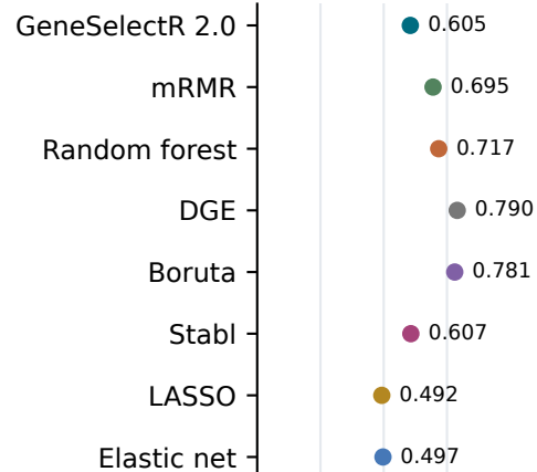
Asthma
