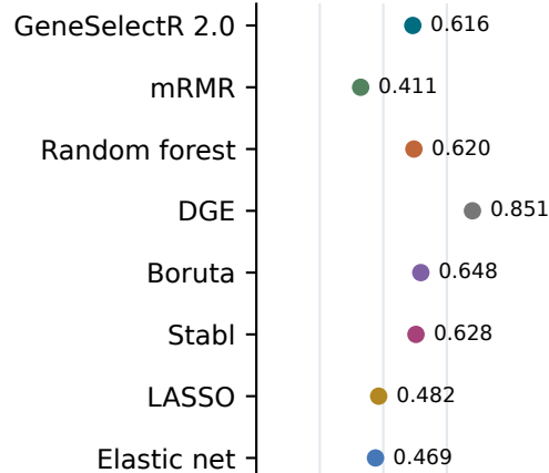
IMvigor210
