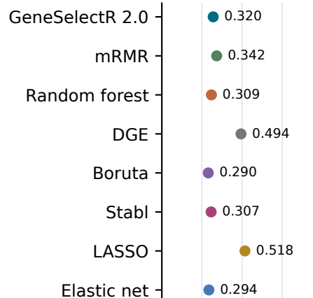
IMvigor210
