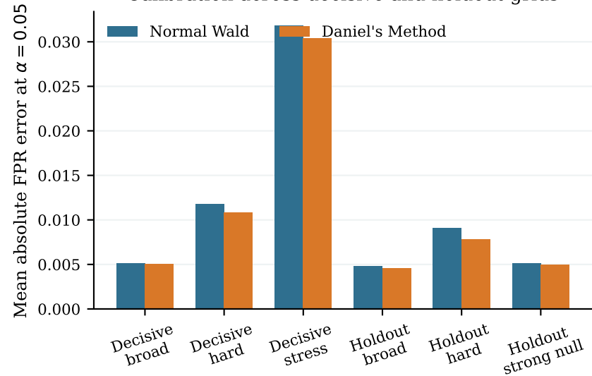
Calibration across decisive and holdout grids
