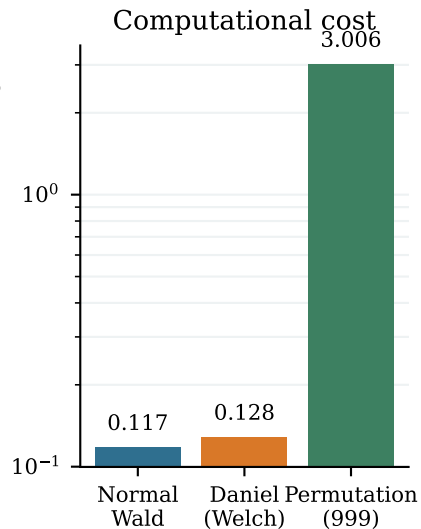
Computational cost
