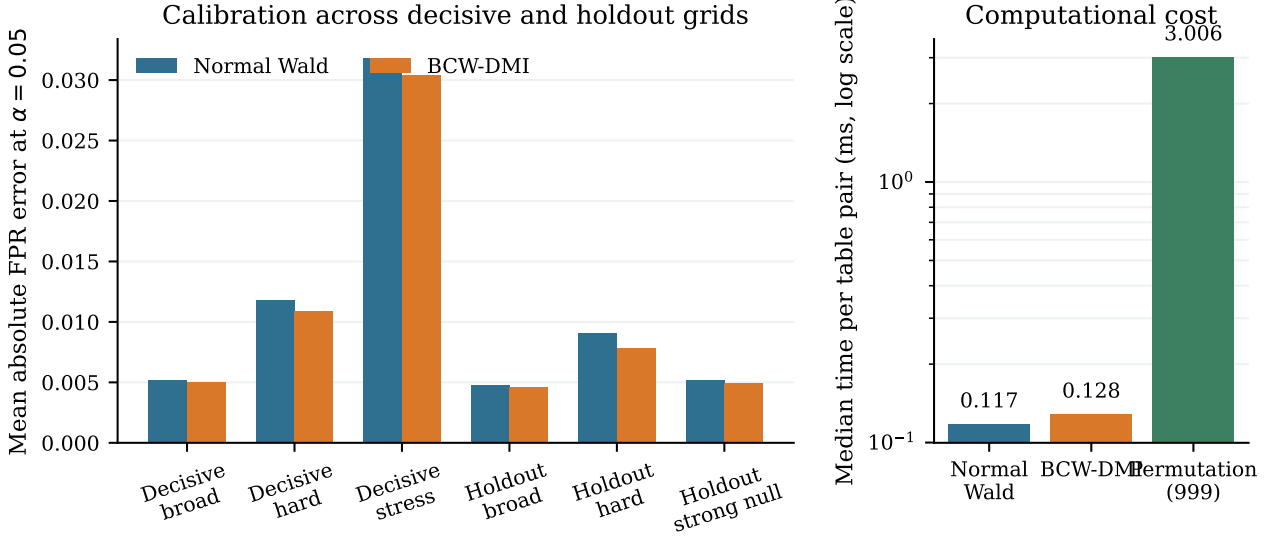
Figure 3: Accuracy and cost summary. Left: normal and BCW-DMI MAE across the decisive study and independent holdout. The largest benefit occurs in deliberately liberal hard regimes; broad and strong-null effects are small. Right: median observed single-pair runtime on a logarithmic scale. The permutation result uses 999 optimized table permutations and is not JIDT’s one-table independence shuffle.
