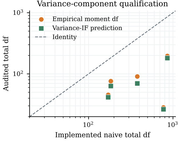
Figure 4: The implemented degrees of freedom are heuristic. Empirical moment degrees of freedom for the total estimated variance are well below Eq. (12). A variance-functional influence calculation tracks the audit more closely. The current procedure must therefore be described as Welch-inspired, not exact.
