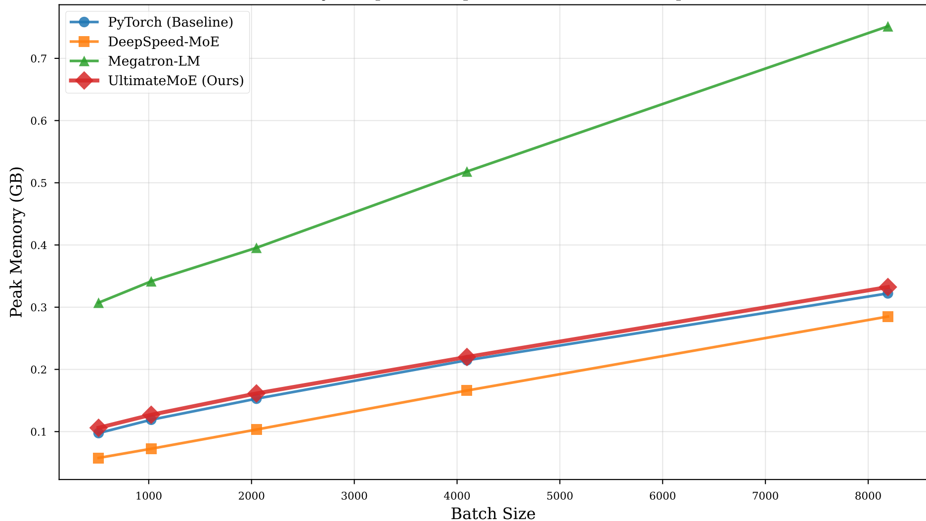
Memory Footprint Comparison (8 GPUs, 128 Experts)
