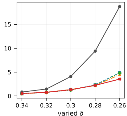
(c) Chess (fixed \gamma=62\% )
