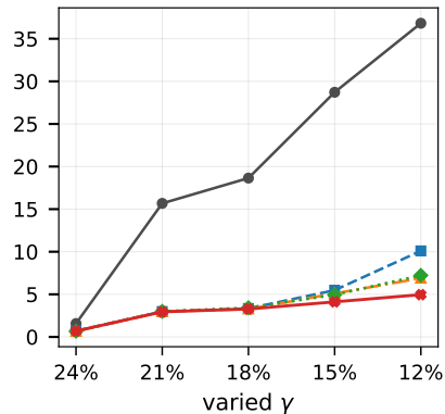
(b) Mushroom (fixed \delta=0.3 )
