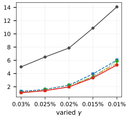
(e) BMS2 (fixed \delta=0.3 )
