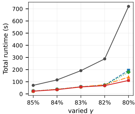
(a) Connect (fixed \delta=0.3 )
