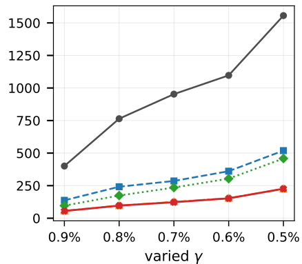
(f) T40I10D300K (fixed \delta=0.3 )
