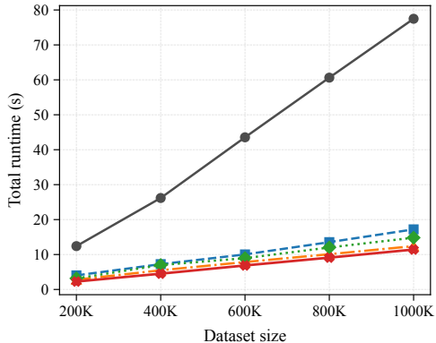
(a) Runtime under fixed \gamma=0.05\% and fixed \delta=0.25 .
