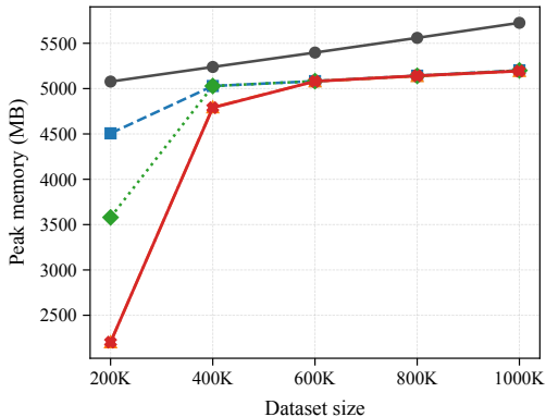
(b) Memory under fixed \gamma=0.05\% and fixed \delta=0.25 .
