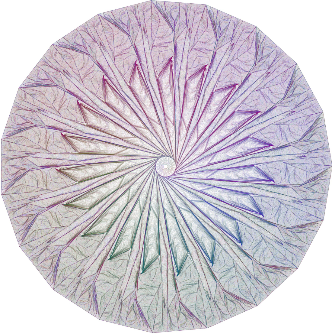
Figure 1: One of the seven 19-curve diagrams (certificate fc7ad34 ), drawn from its certificate at near-uniform crossing density by the plotter described in the data repository: 19 curves, 524,286 crossings, every one of the 524,288 regions present exactly once. The centre hole is the region inside all 19 curves; the outer face is the region outside all of them. Colours identify curves.
