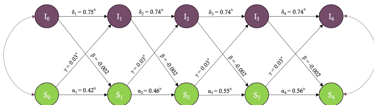
FIGURE 3. Cross-lagged panel models showing associations between social media use and inattention symptoms. All coefficients are standardized \beta weights.
