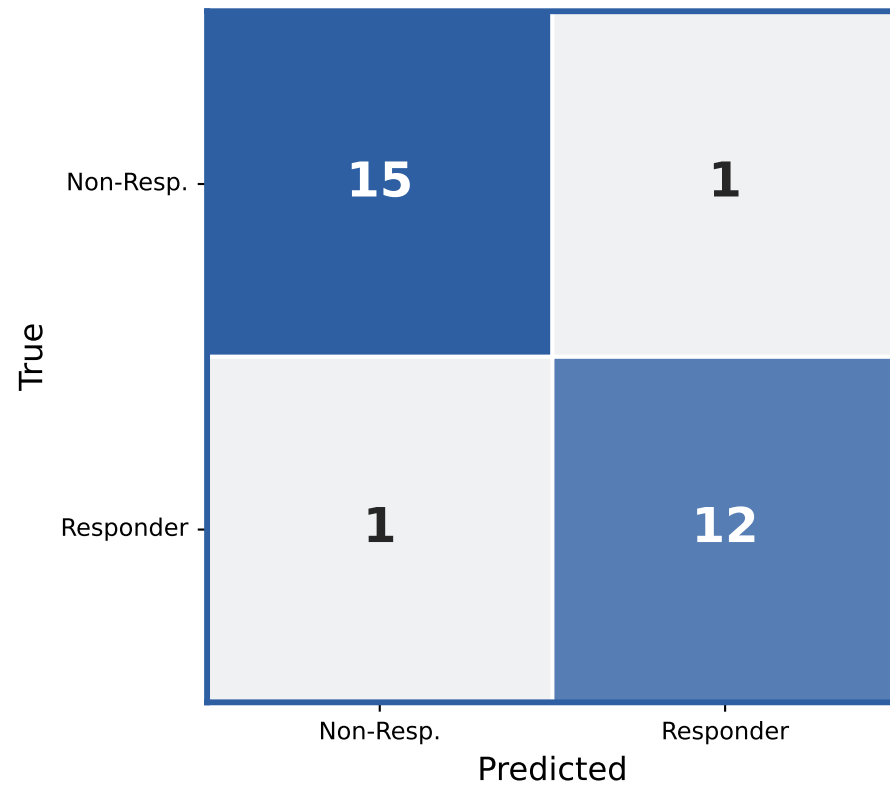
GradientBoosting Acc=0.931 F1=0.923
