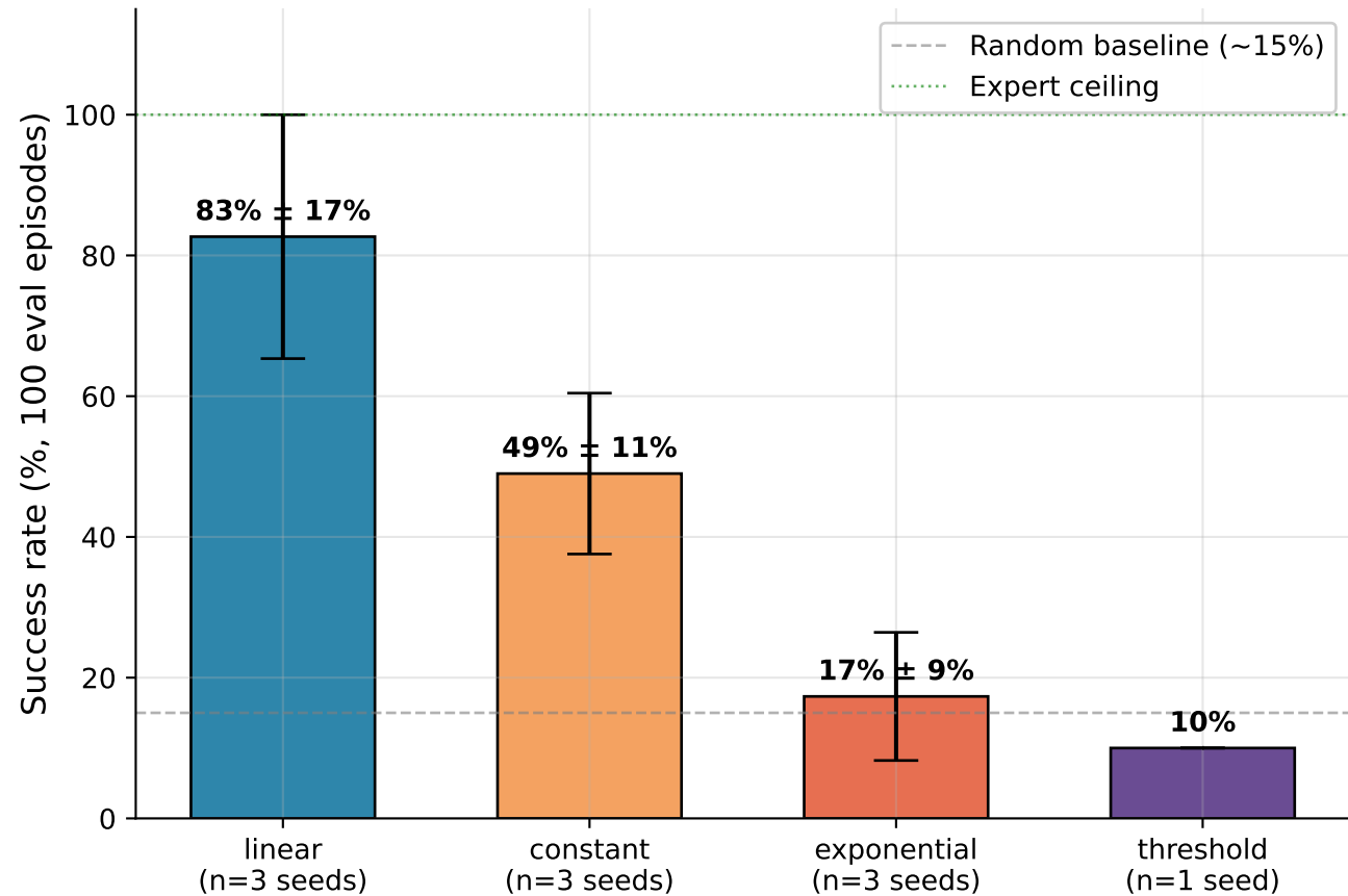
DAGger \beta -Schedule Ablation (init 100 demos)
