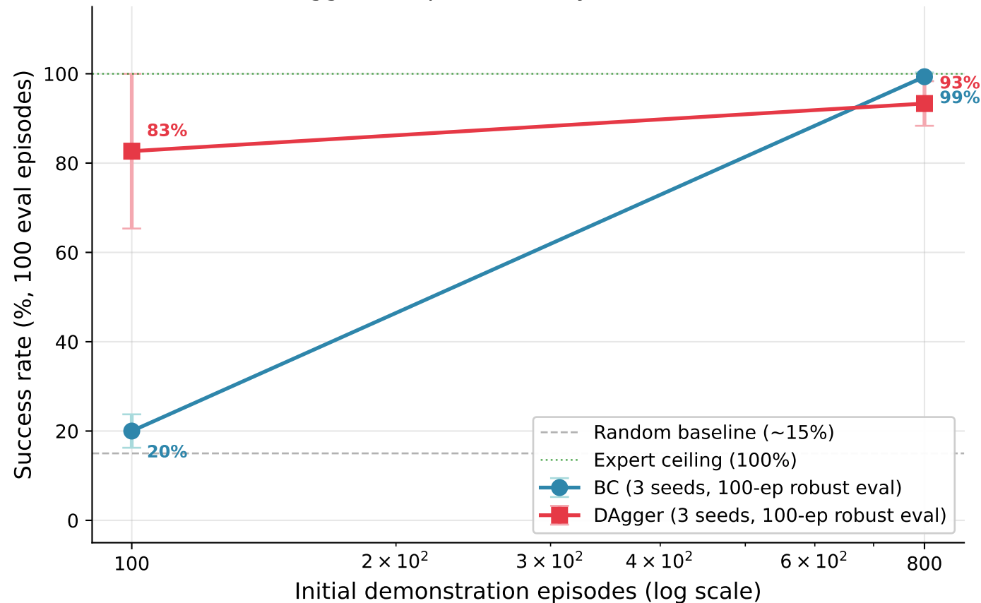
BC vs DAgger Sample Efficiency — FetchPickAndPlace
