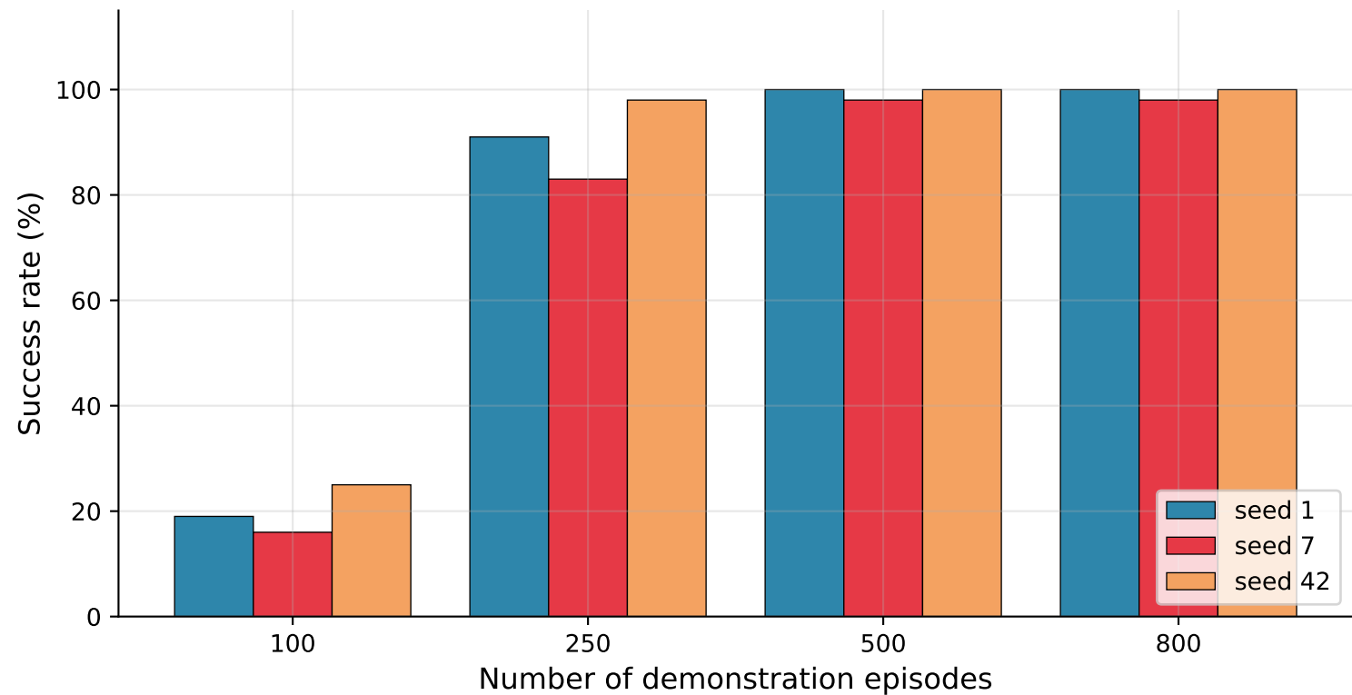
Per-Seed Variance Across Demo Counts
