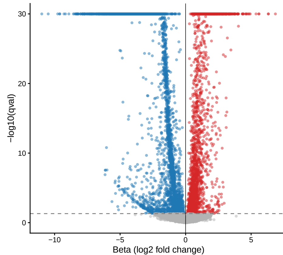
pmk1 vs Guy11M | 24H
