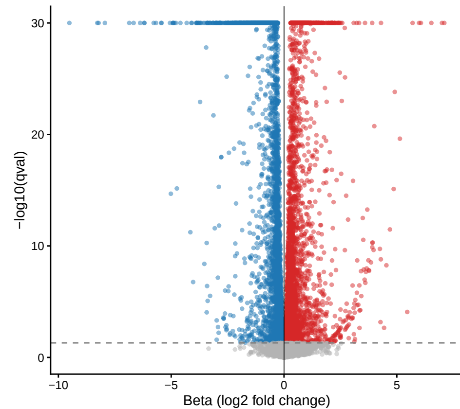
pmk1 vs Guy11M | 4H
