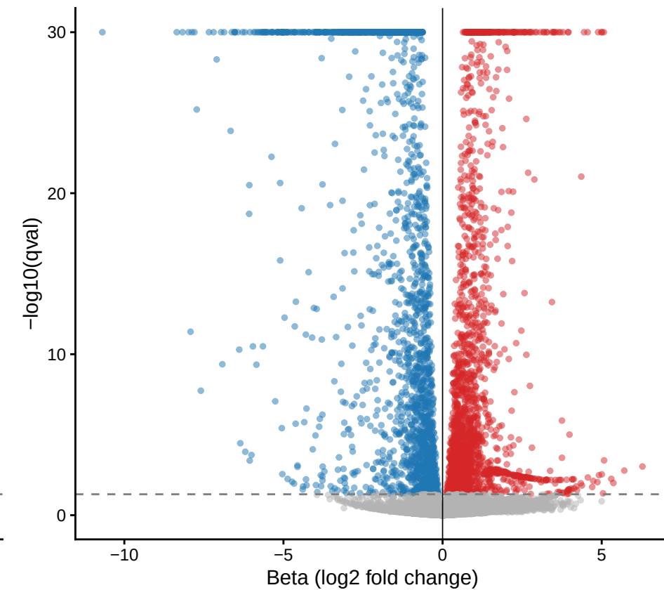
pmk1 vs Guy11M | 2H
