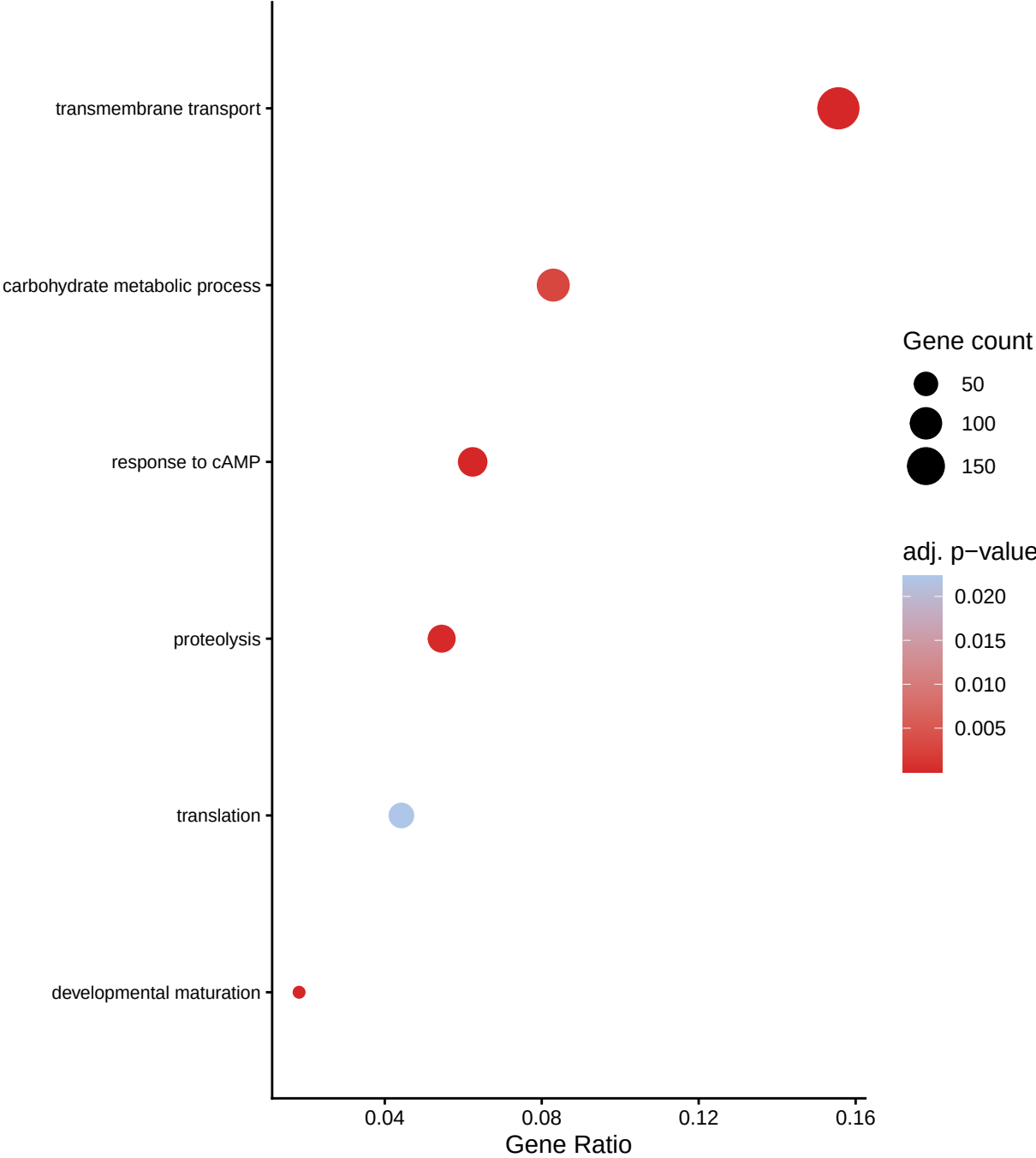
pmk1 vs Guy11M | 24H | downregulated | BP
