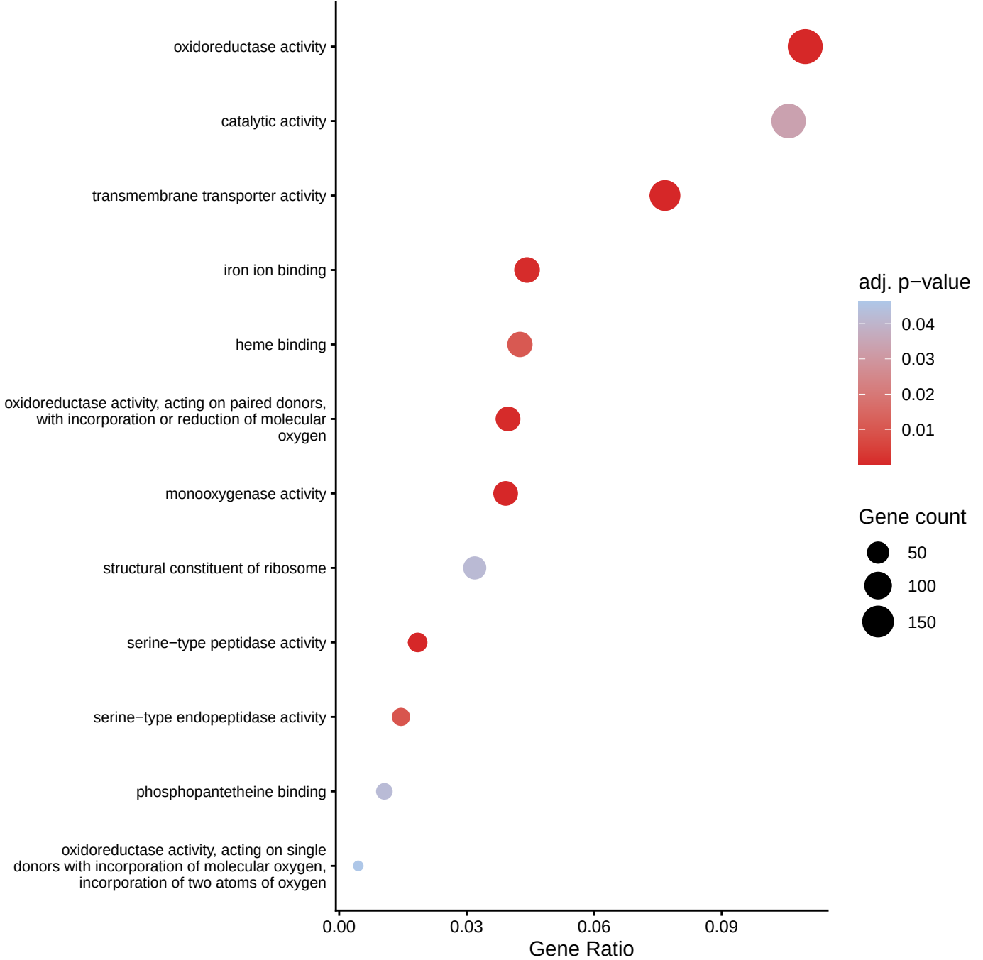
pmk1 vs Guy11M | 24H | downregulated | MF
