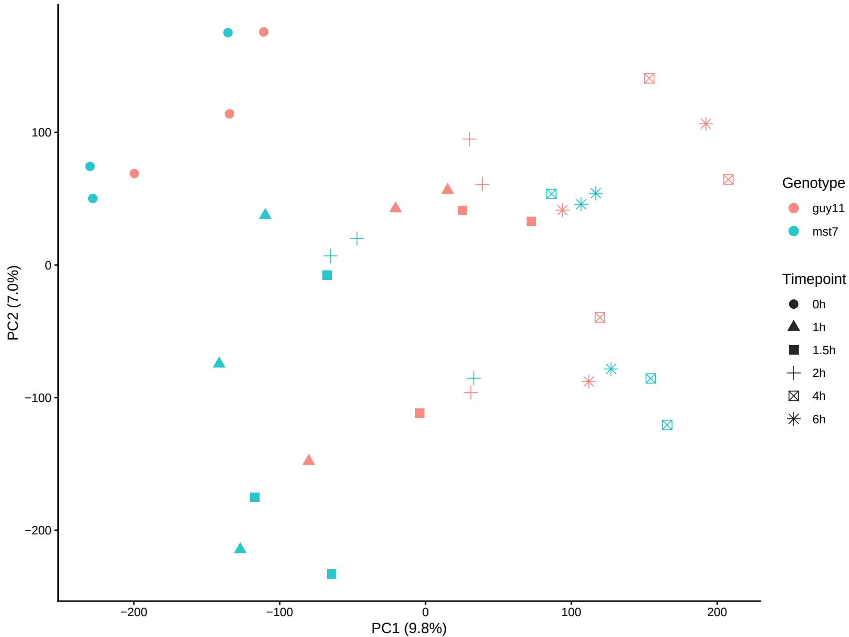
MST7 PCA of phosphosite abundances
