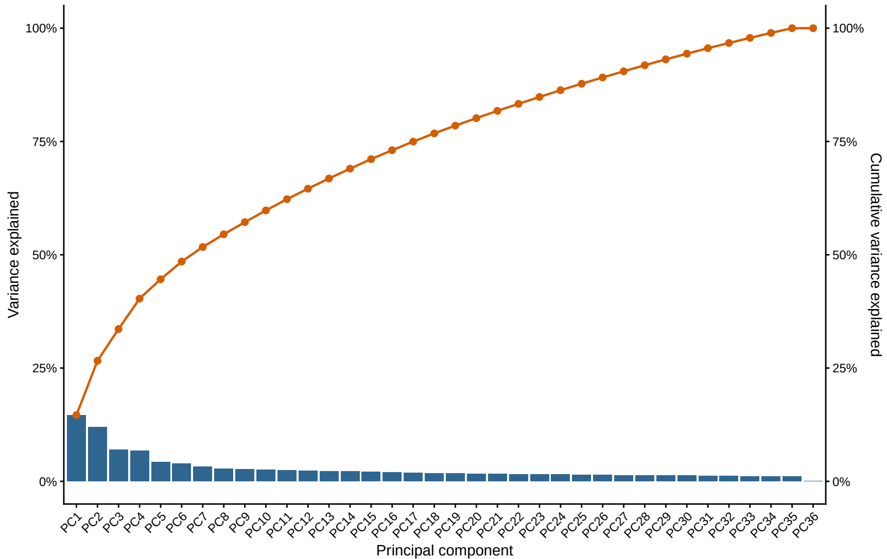
PMK1 PCA variance explained
