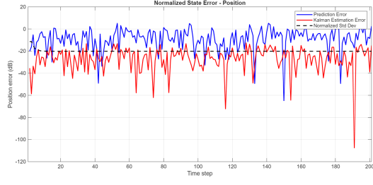
Figure 2.8: State estimation comparison with R_n = 100R_{n_{\text{true}}}
