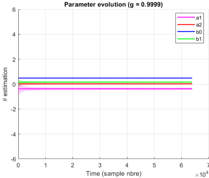
Figure 1.5: Uncertainty variation - Low LTI system ( g=0.9999 )
