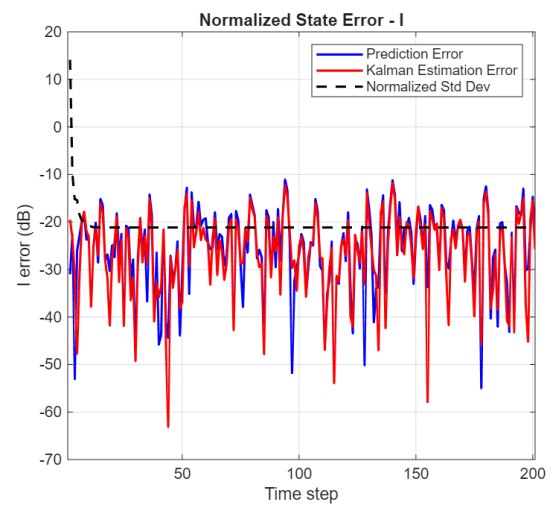
Figure 2.8: State estimation comparison with R_n = 100R_{n_{\text{true}}}
