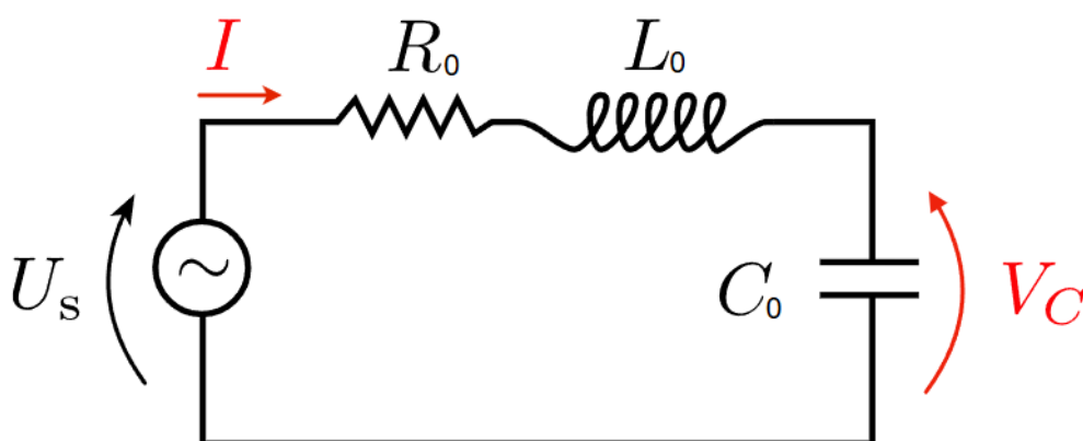
Figure 2.1: Studied RLC circuit
