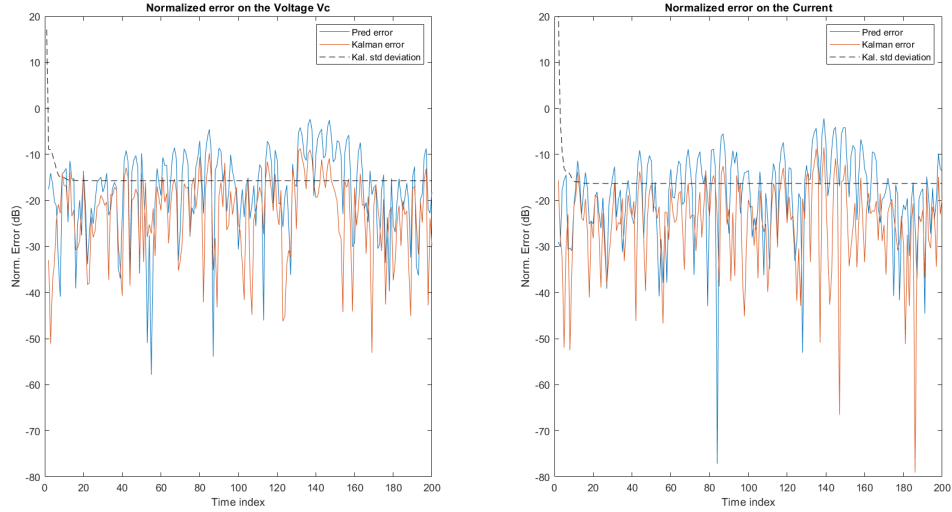
Figure 2.10: State estimation comparison with R_n = 100R_{n_{\text{true}}}
