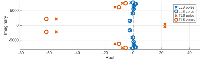
Fig. 10. Poles and zeros of the LLS and TLS estimators
