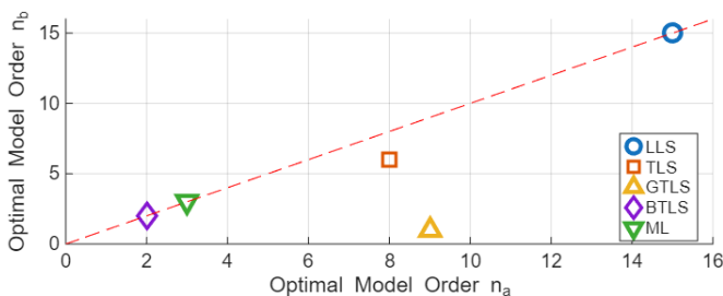
Fig. 9. Optimal orders for each estimator, according to the AIC criterion. The red dashed line is the stability limit n_a = n_b
