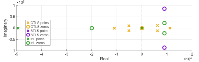
Fig. 11. Poles and zeros of the GTLS, BTLS and ML estimators
