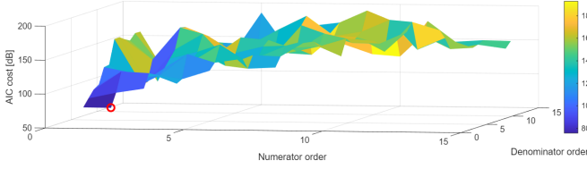
Fig. 7. AIC cost depending on the order of the transfer function for the BTLS estimator. The optimal order is circled in red.
