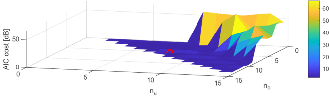
Fig. 8. AIC cost depending on the order of the transfer function for the TLS estimator. The optimal order is circled in red.
