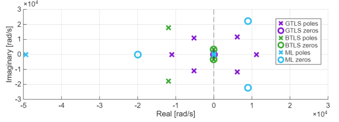
Fig. 12. Poles and zeros of the GTLS, BTLS and ML estimators.
