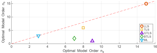
Fig. 10. Optimal orders for each estimator, according to the AIC criterion. The red dashed line is the stability limit n_a = n_b .
