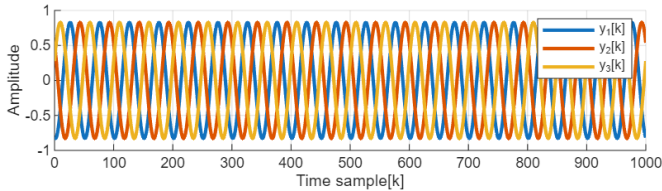
Fig. 10. Three-phased signal measured by 3 (faultless) sensors.
