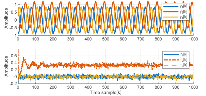
Fig. 9. Measured signal (top) and residuals(bottom).
