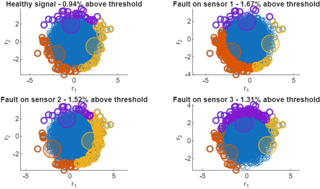
Fig. 6. Residuals (blue) and fault directions: F_1 in orange, F_2 in yellow and F_3 in purple. Residuals above the threshold are colored with the fault they are attributed to.
