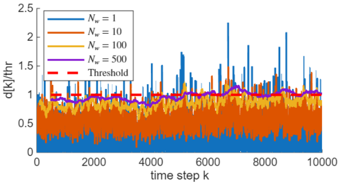
Fig. 7. Decision variable depending on the window length for a fault occurring from sample 5000 until the last sample. d[k] is scaled by their threshold such that their overlapping has a meaning.
