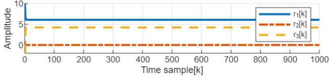
Fig. 9. Residuals with the alternative incidence matrix.
