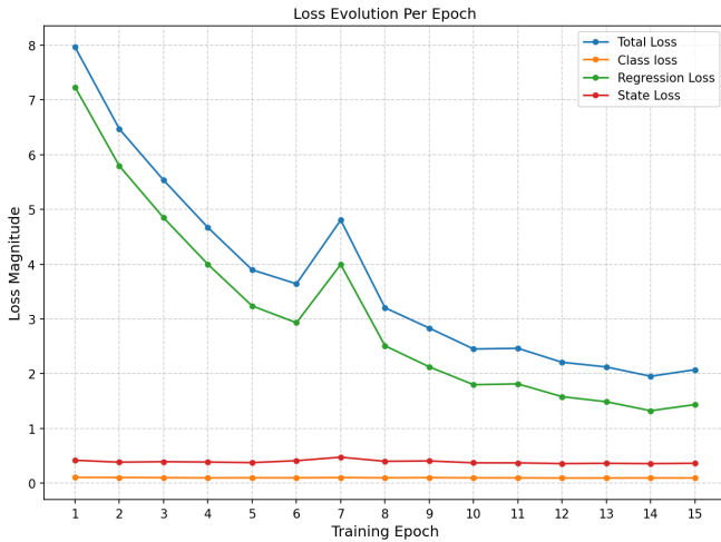
Fig. 9: Evolution of the loss during training.
