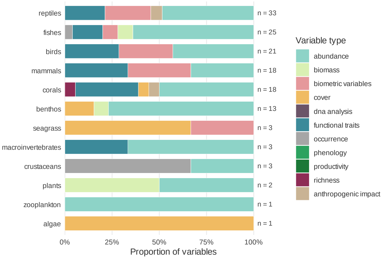
(B) Marine
