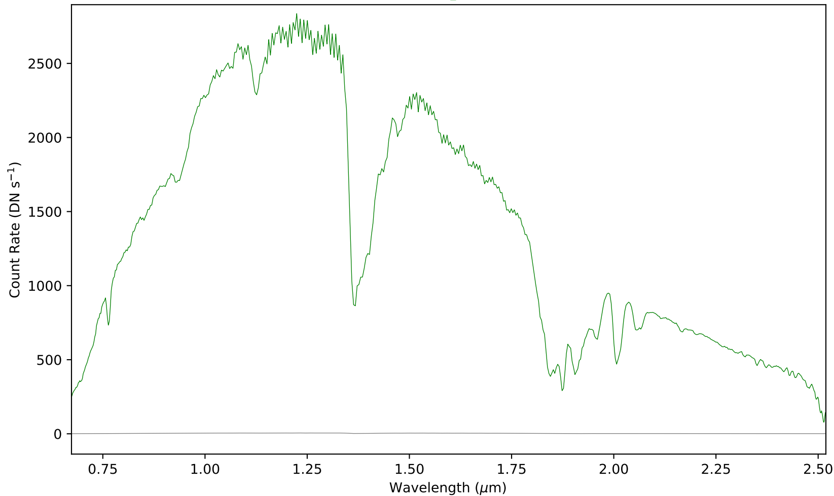
combspec34-35.fits - Aperture 1
