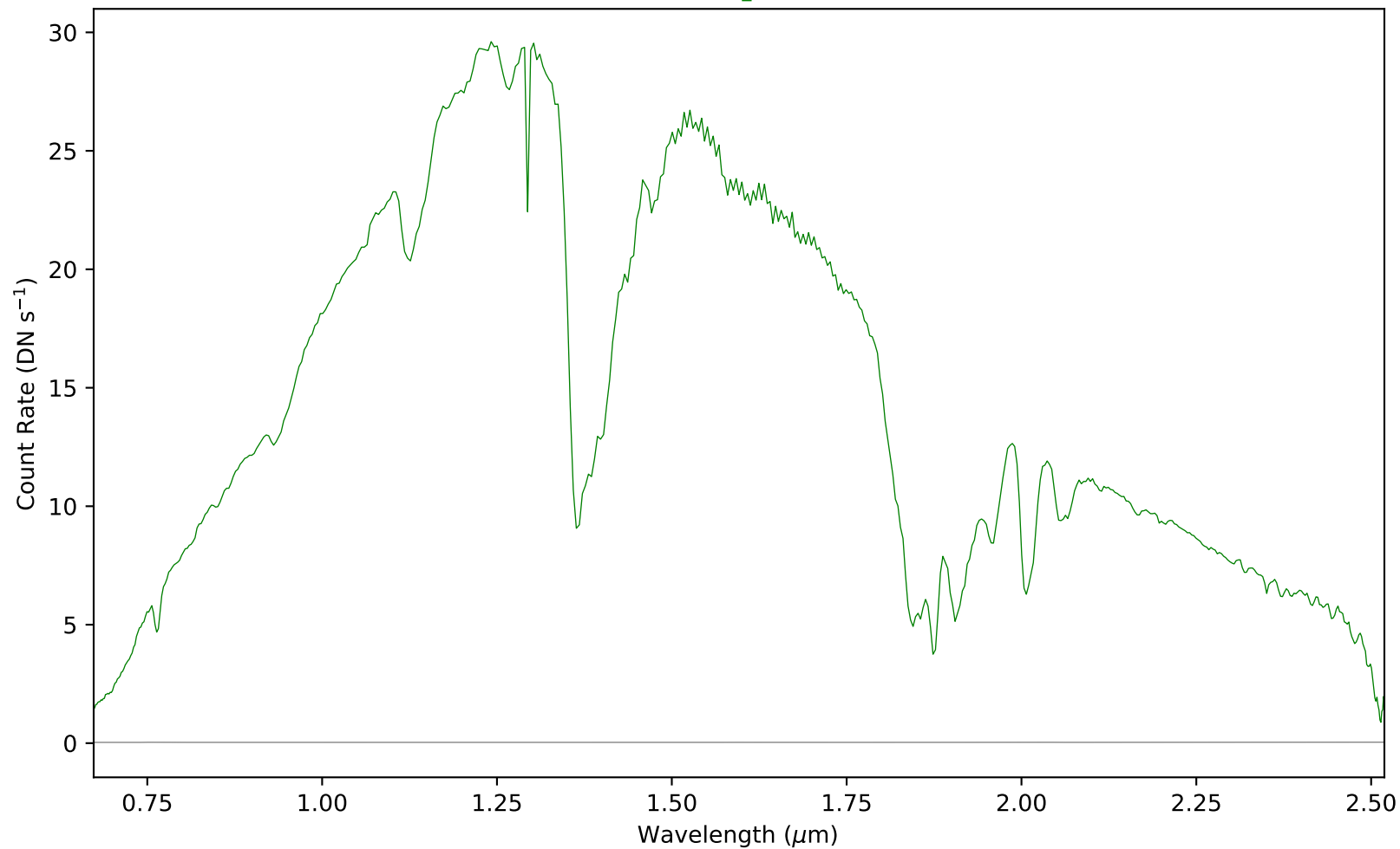
combspec36-53.fits - Aperture 1
