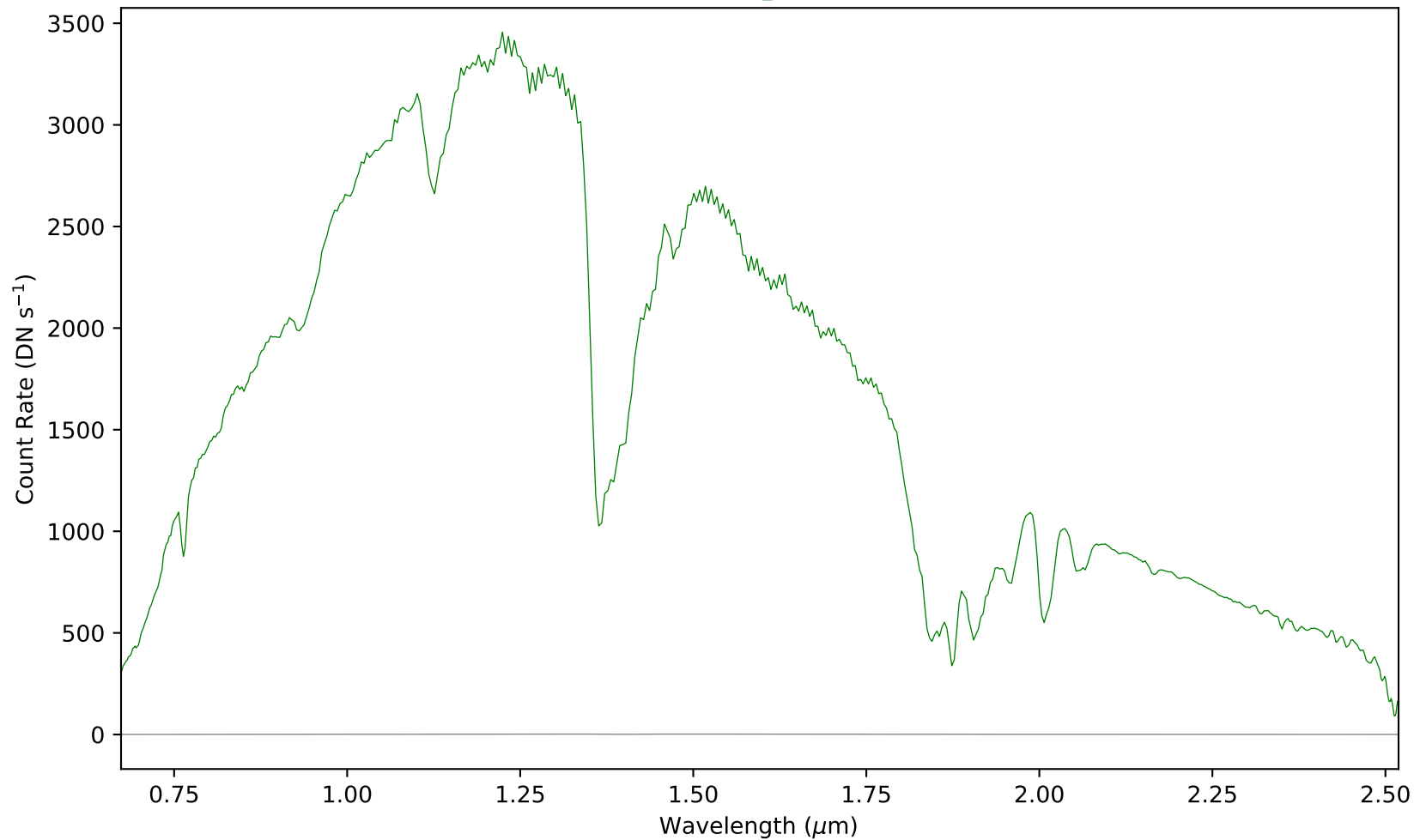
combspec44-55.fits - Aperture 1
