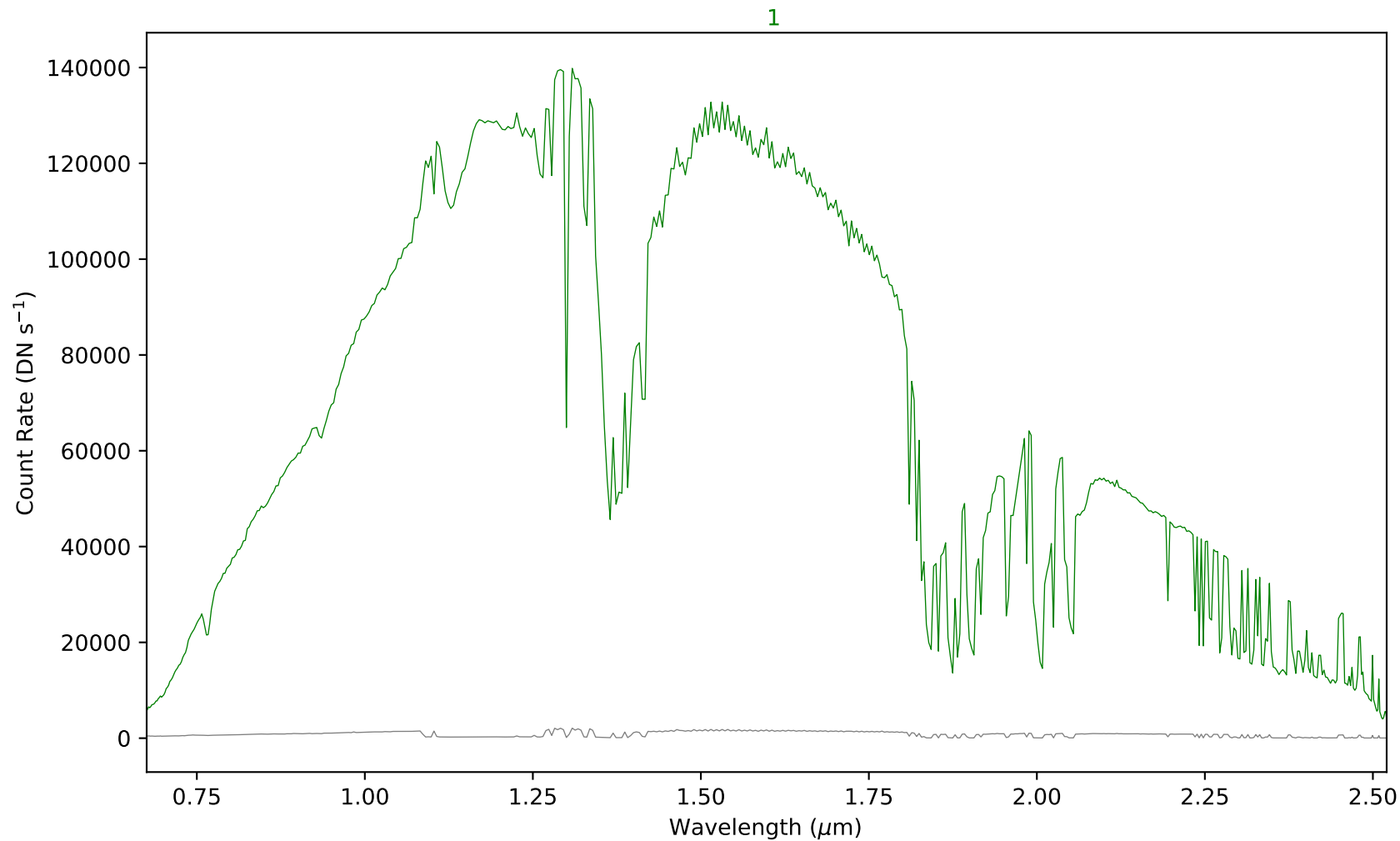
combspec11-249.fits - Aperture 1
