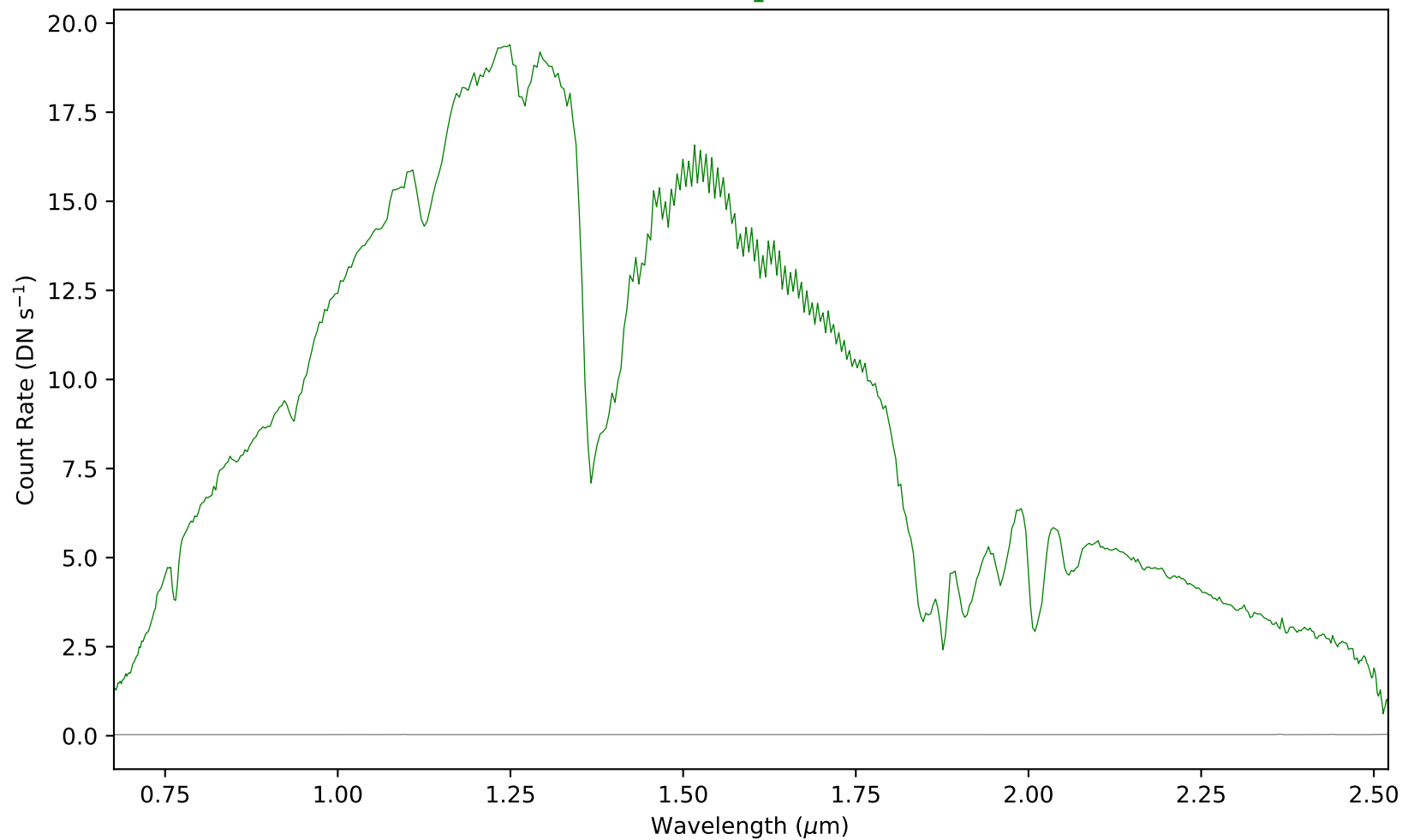
combspec198-211.fits - Aperture 1
