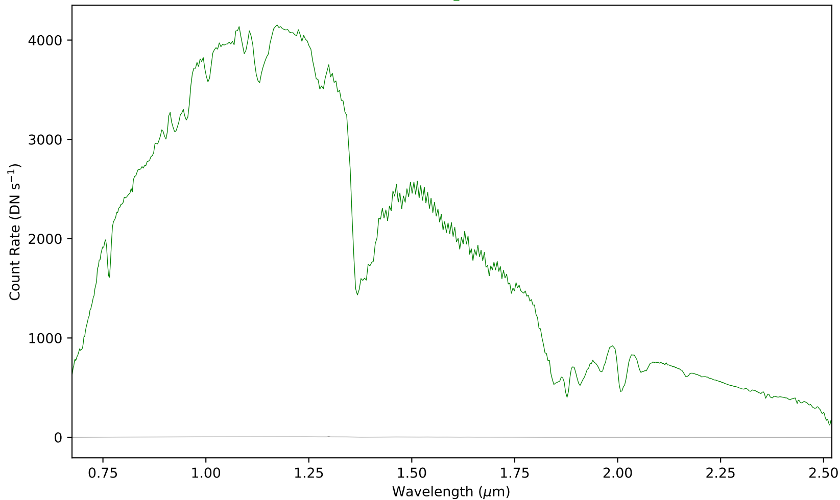
combspec61-104.fits - Aperture 1
