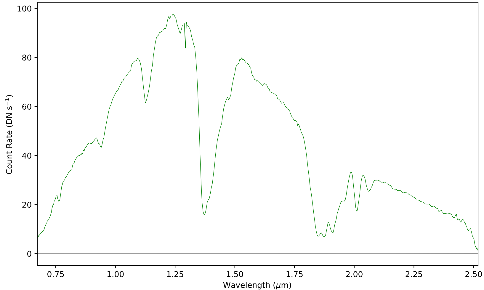
combspec19-32.fits - Aperture 1
