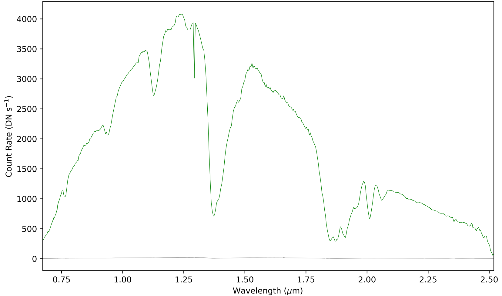
combspec33-42.fits - Aperture 1
