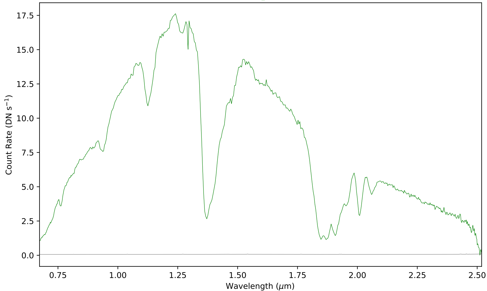
combspec59-66.fits - Aperture 1
