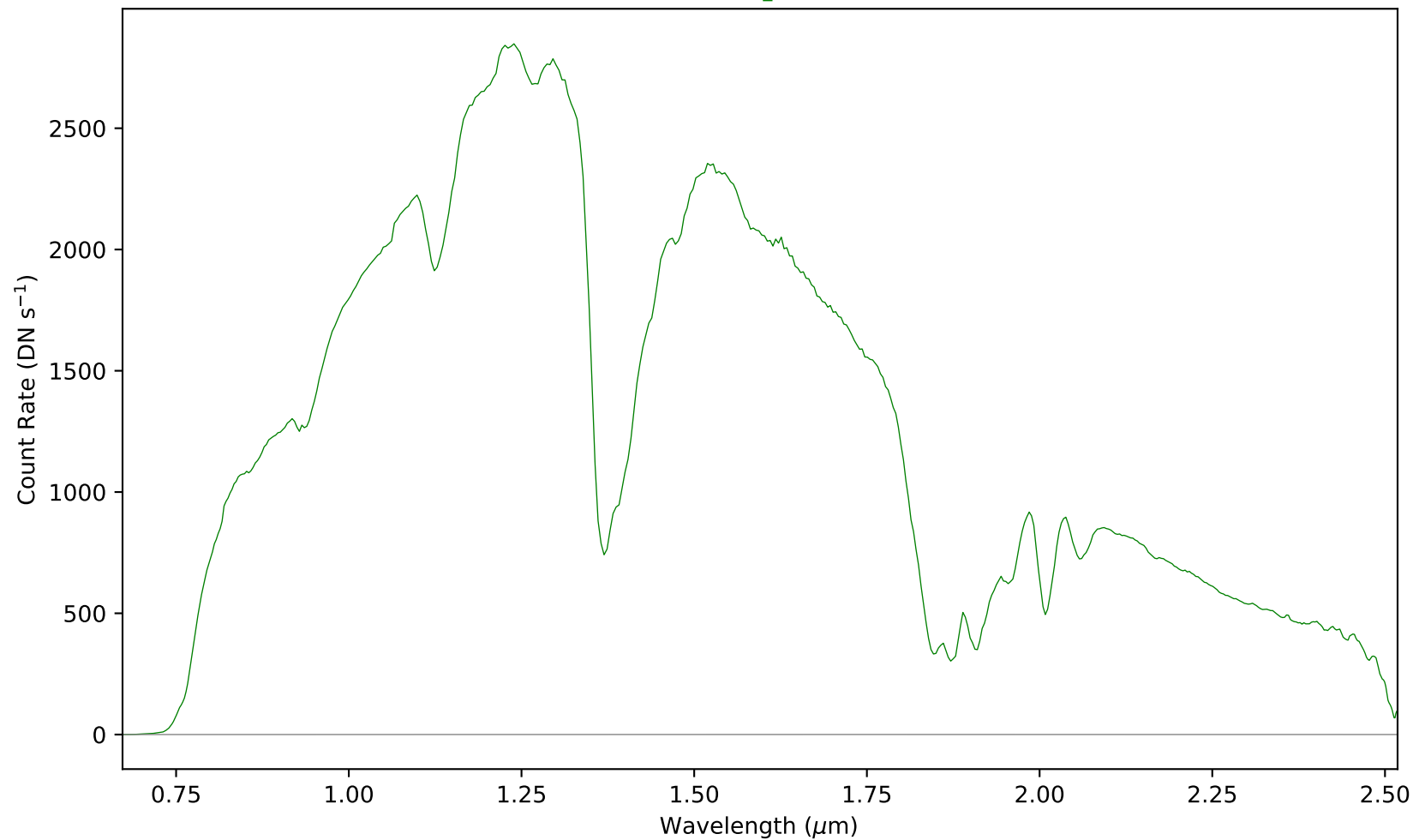
combspec1038-1047.fits - Aperture 1
