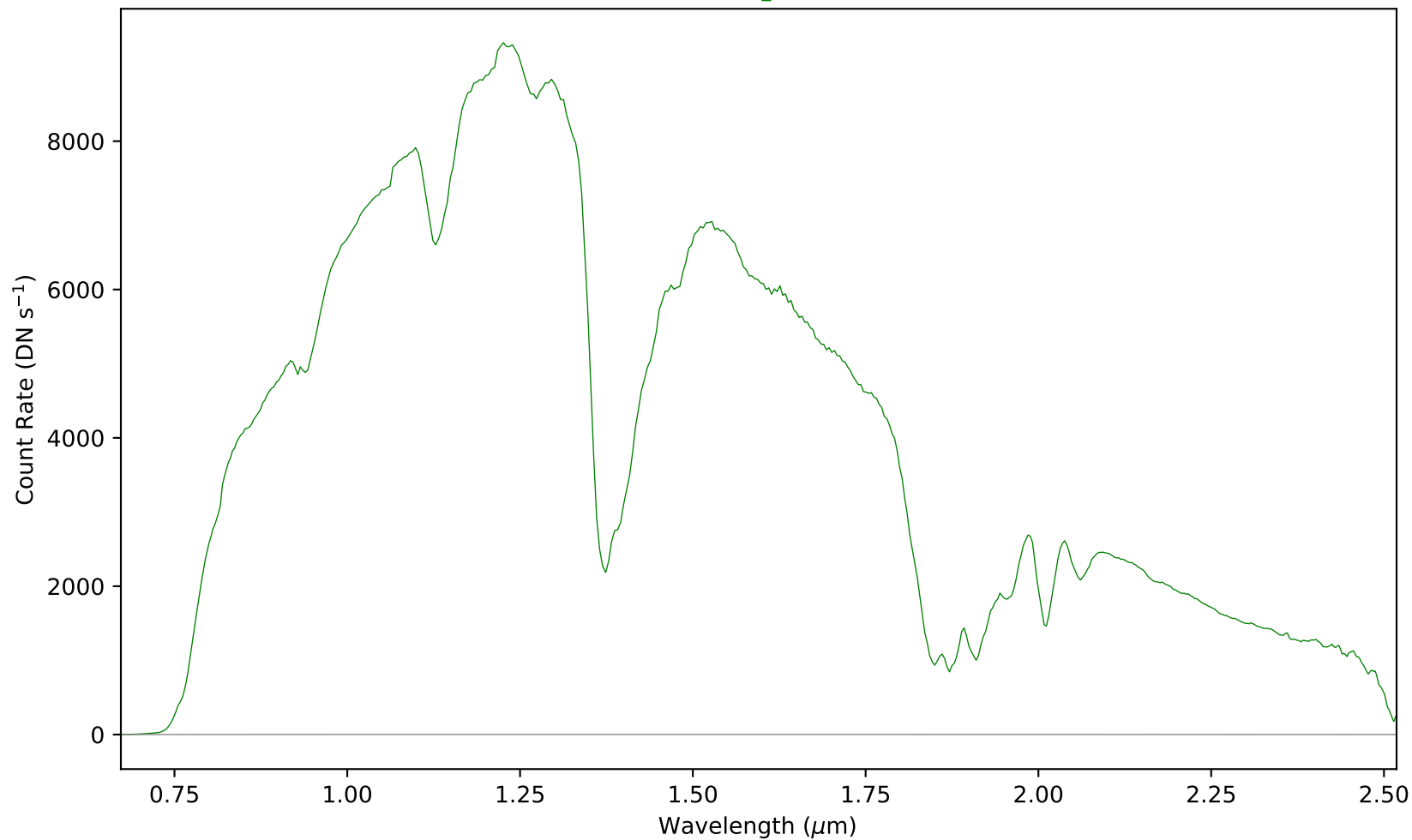
combspec1048-1057.fits - Aperture 1
