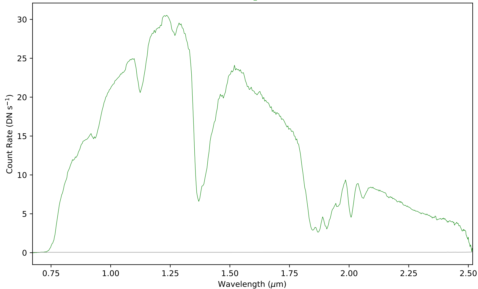
combspec1058-1071.fits - Aperture 1
