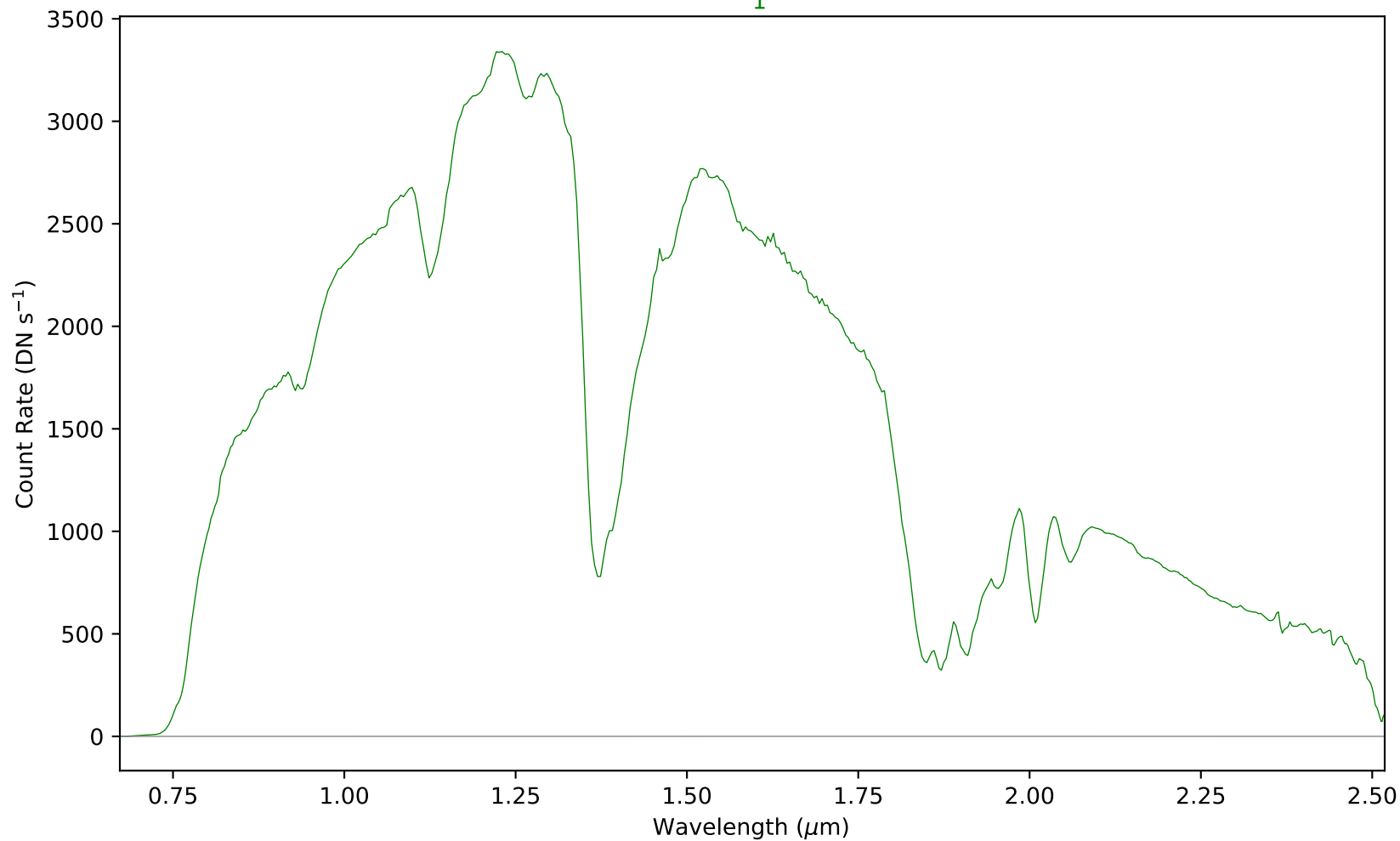
combspec1098-1107.fits - Aperture 1
