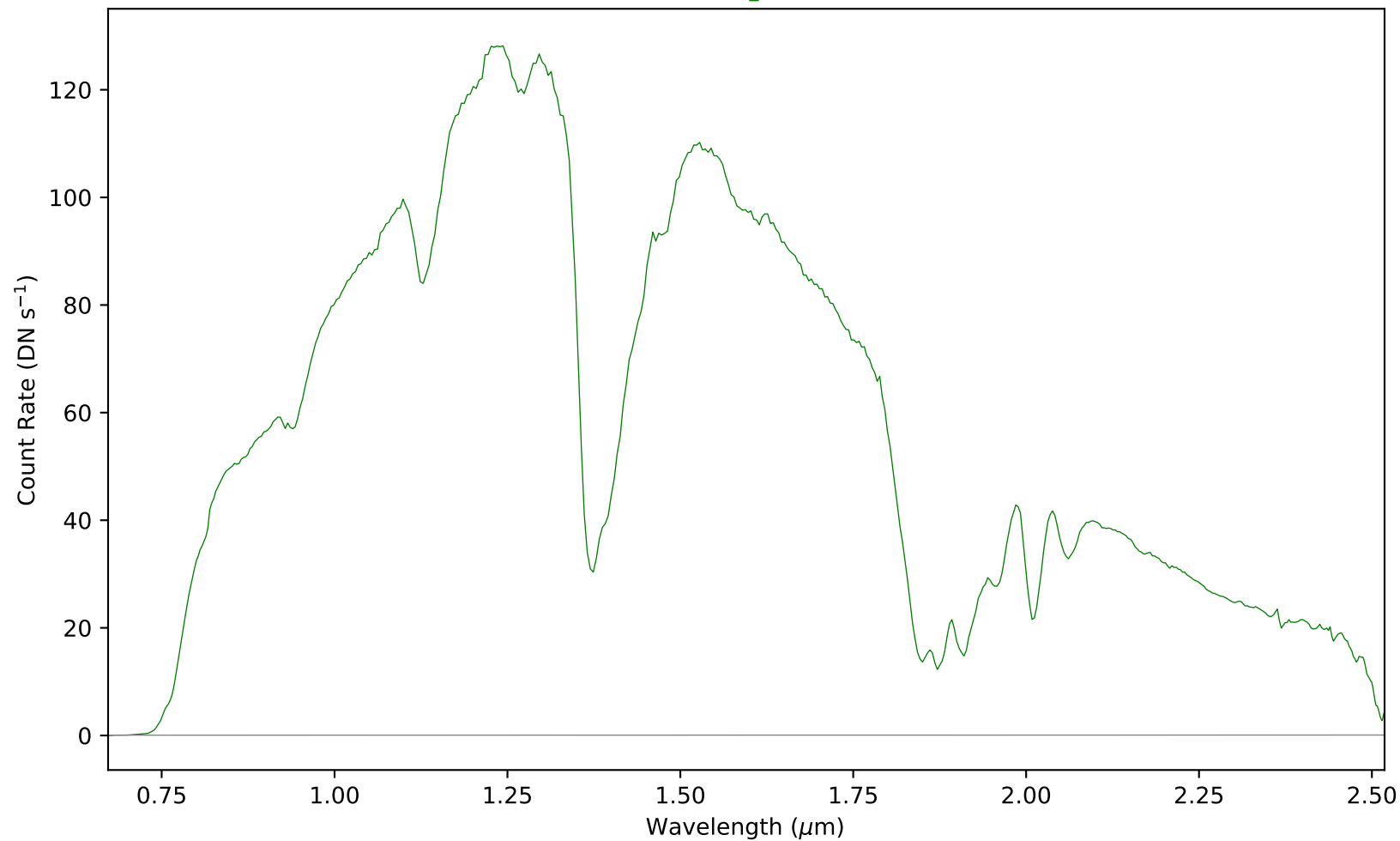
combspec1108-1117.fits - Aperture 1
