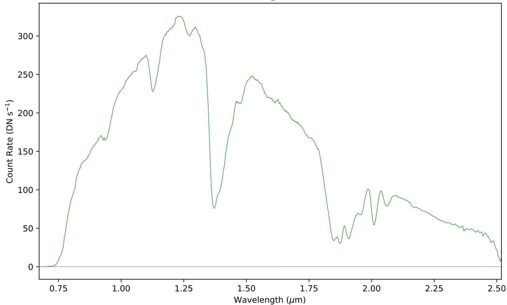
combspec1118-1127.fits - Aperture 1
