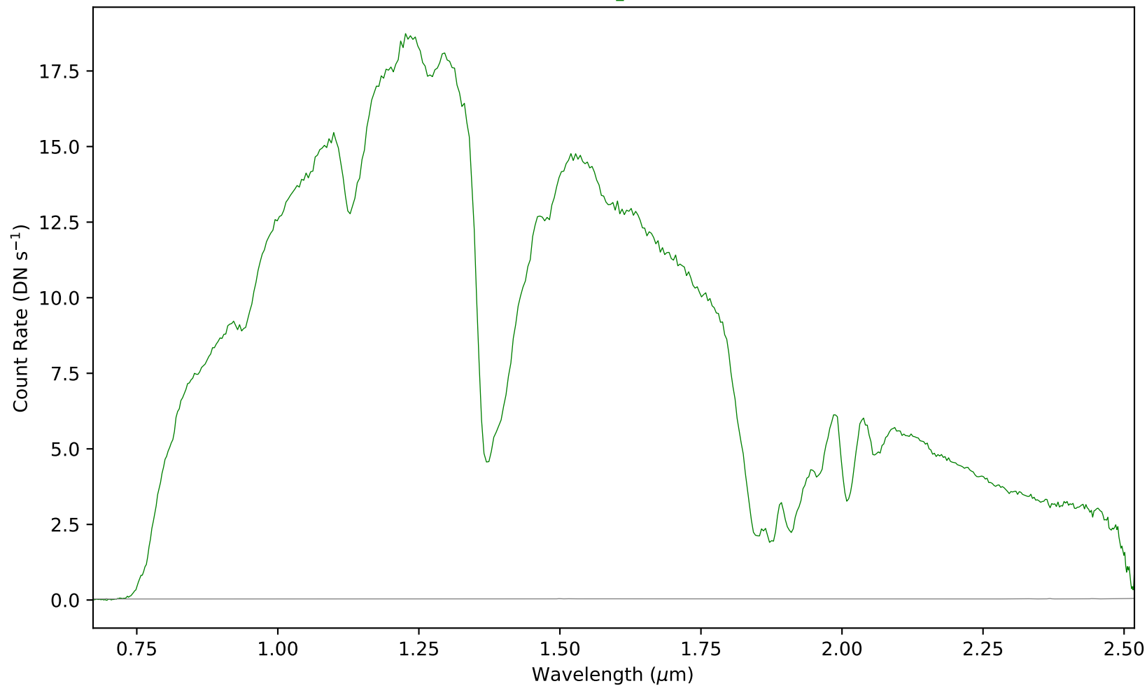
combspec1128-1141.fits - Aperture 1
