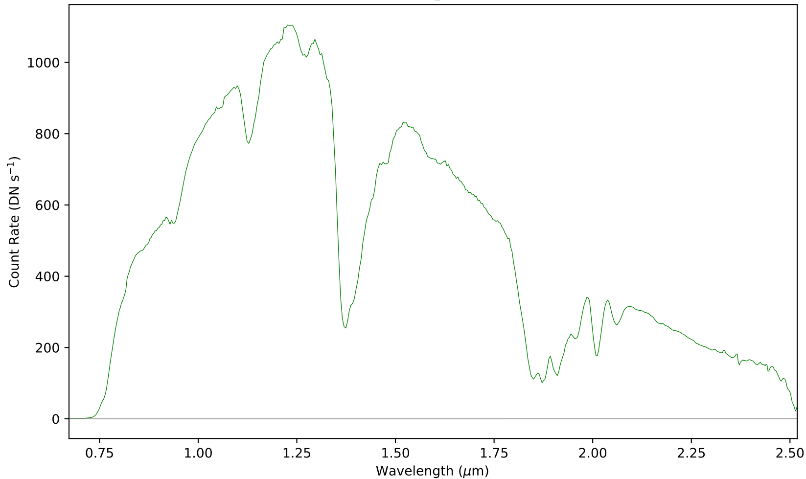
combspec1158-1171.fits - Aperture 1
