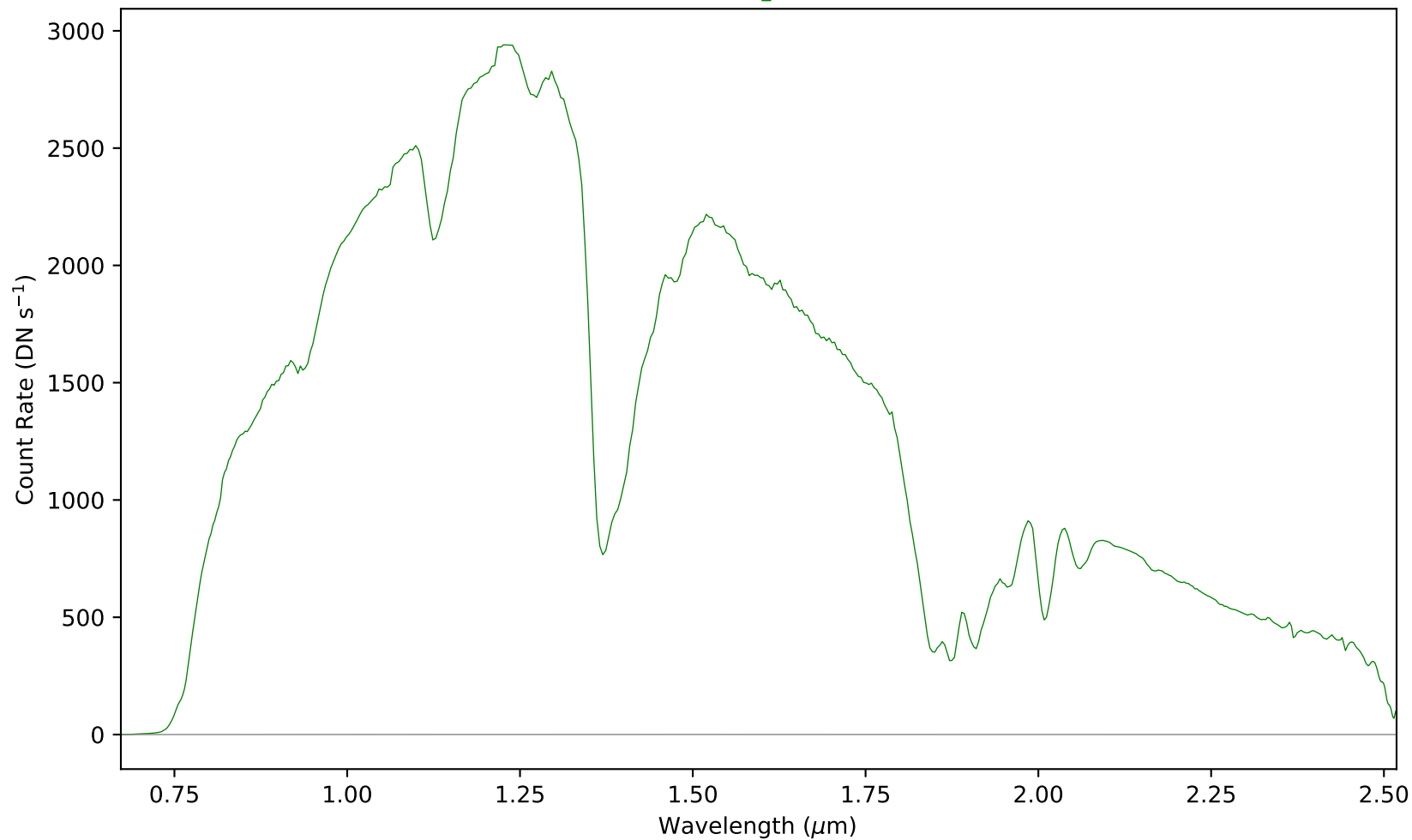
combspec1172-1181.fits - Aperture 1
