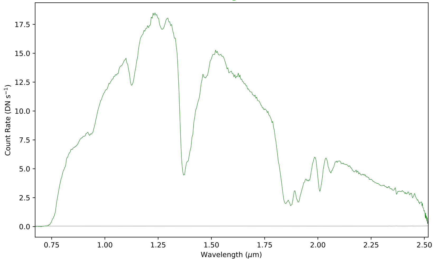
combspec1196-1209.fits - Aperture 1
