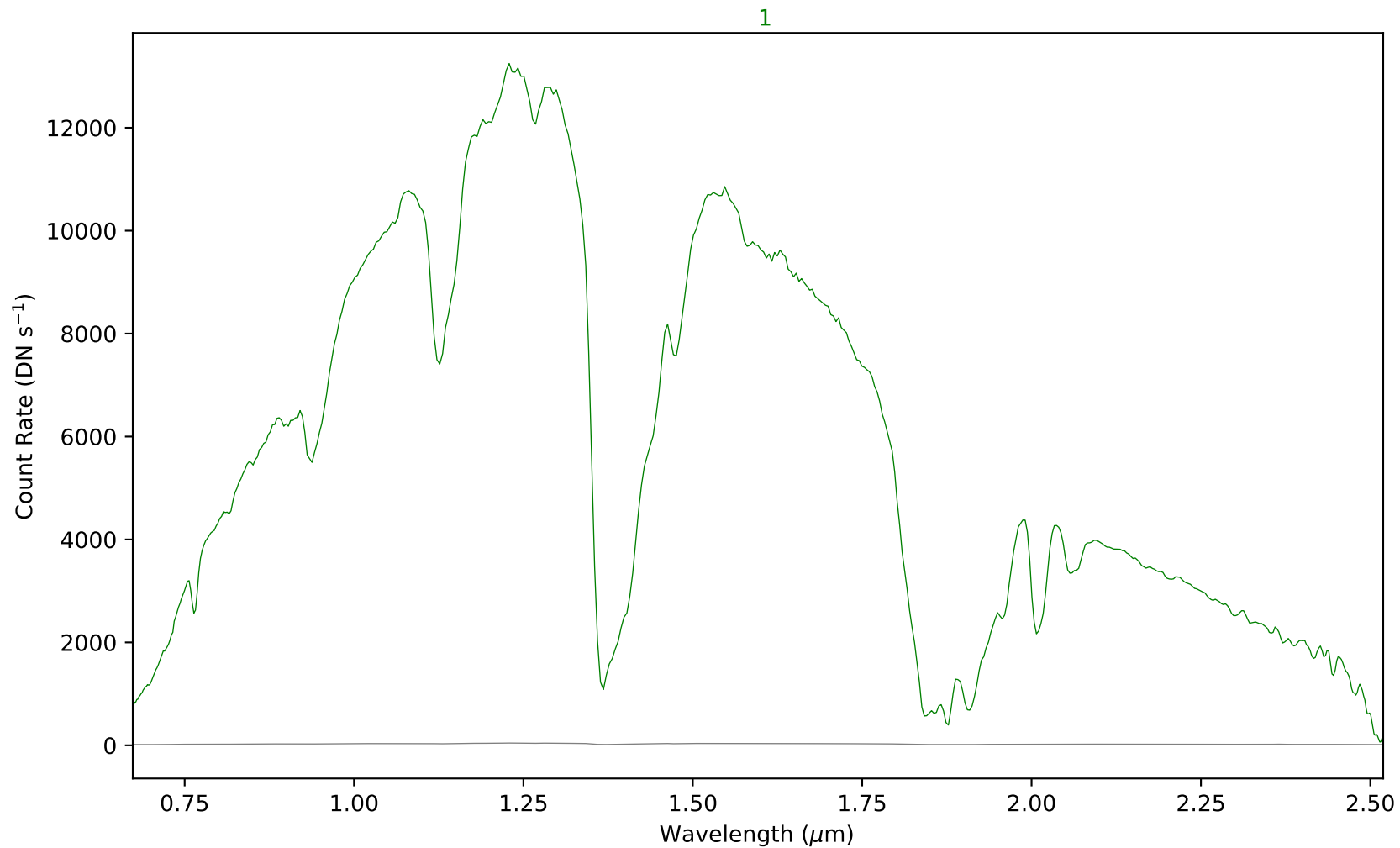
combspec134-311.fits - Aperture 1
